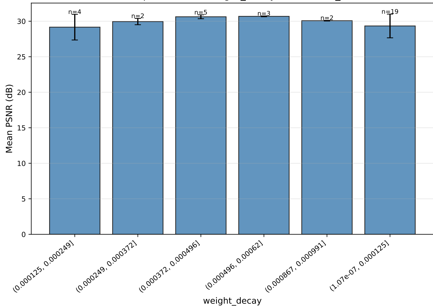
Mean PSNR per value of weight_decay — DHTCUN_baseline
